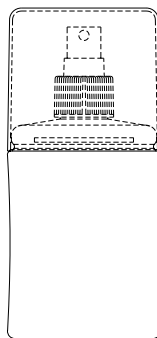
NO-48 / PET 250 C.C. 71.6 mm (L) 50.3 mm (W) 154.8 mm (H)
