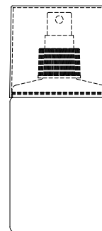
NO-97 / PET 200 C.C. 64.8 mm (L) 46.2 mm (W) 148.4 mm (H)
