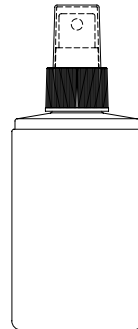
NO-80A / PET 200 C.C. Ø 57.5 mm (L) 142.9 mm (H)
