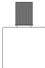
NO-27 / PVC 15 C.C. 42.5 mm (L) 16.5 mm (W) 64.2 mm (H)
