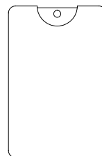
NO-121 / PET 20 C.C. 55.8 mm (L) 10.8 mm (W) 86.8 mm (H)
