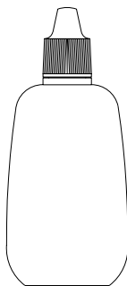
NO-9 / LDPE 8 C.C. 38.8 mm (L) 17 mm (W) 89 mm (H)
