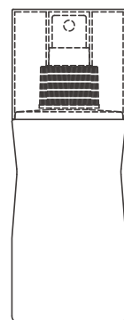
NO-87D / PET 150 C.C. 53 mm (L) 43 mm (W) 145.5 mm (H)
