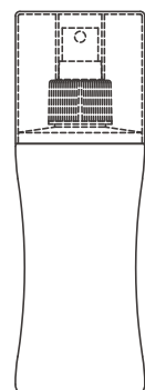
NO-89 / PET 200 C.C. Ø 57 mm (L) 168 mm (H)
