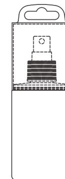
NO-128 / PET 200 C.C. Ø 57.5 mm (L) 168.1 mm (H)
